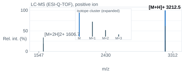
Fig. 2 — ESI-Q-TOF mass spectrum; base peak [M+H] + 3212.5 m/z.
