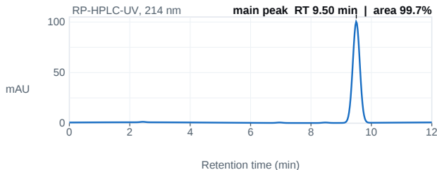
Fig. 1 — HPLC chromatogram; main peak 9.50 min, 99.7% area.
