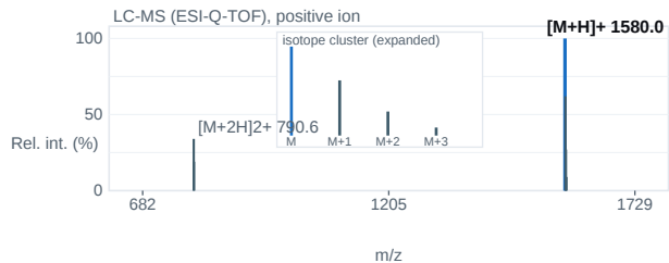
Fig. 2 — ESI-Q-TOF mass spectrum; base peak [M+H] + 1580.0 m/z.
