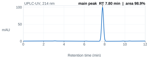
Fig. 1 — UPLC chromatogram; main peak 7.80 min, 98.9% area.
