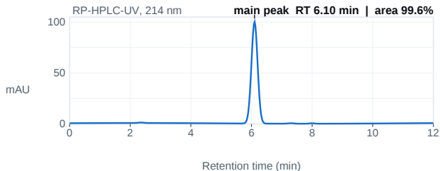
Fig. 1 — HPLC chromatogram; main peak 6.10 min, 99.6% area.
