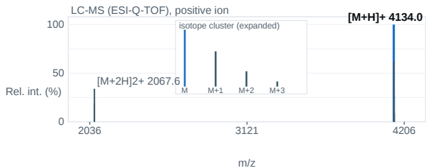
Fig. 2 — ESI-Q-TOF mass spectrum; base peak [M+H] + 4134.0 m/z.
