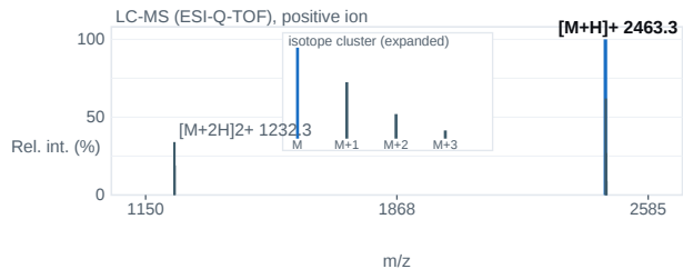
Fig. 2 — ESI-Q-TOF mass spectrum; base peak [M+H] + 2463.3 m/z.
