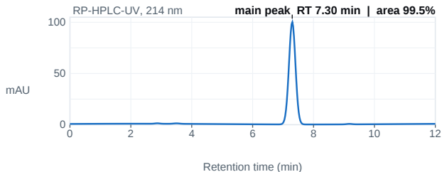
Fig. 1 — HPLC chromatogram; main peak 7.30 min, 99.5% area.
