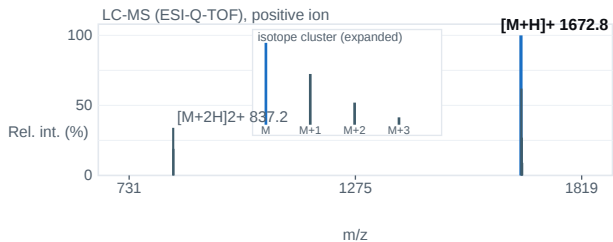
Fig. 2 — ESI-Q-TOF mass spectrum; base peak [M+H] + 1672.8 m/z.
