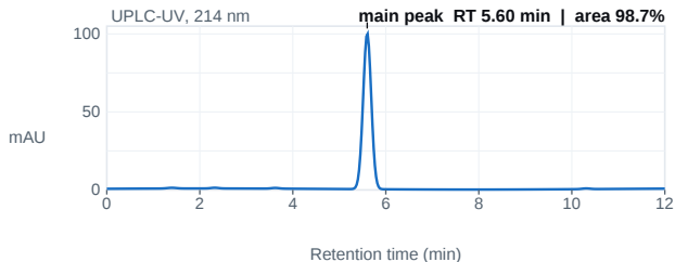
Fig. 1 — UPLC chromatogram; main peak 5.60 min, 98.7% area.
