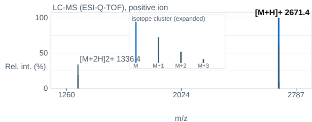
Fig. 2 — ESI-Q-TOF mass spectrum; base peak [M+H] + 2671.4 m/z.
