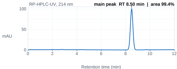
Fig. 1 — HPLC chromatogram; main peak 8.50 min, 99.4% area.
