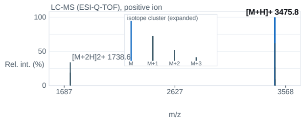
Fig. 2 — ESI-Q-TOF mass spectrum; base peak [M+H] + 3475.8 m/z.
