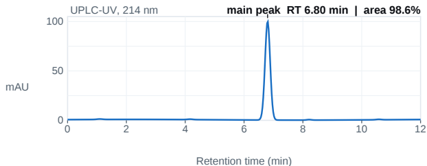
Fig. 1 — UPLC chromatogram; main peak 6.80 min, 98.6% area.
