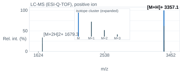
Fig. 2 — ESI-Q-TOF mass spectrum; base peak [M+H] + 3357.1 m/z.
