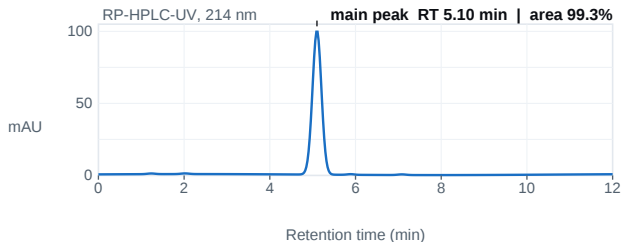
Fig. 1 — HPLC chromatogram; main peak 5.10 min, 99.3% area.
