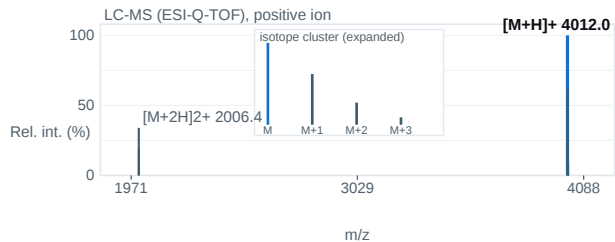
Fig. 2 — ESI-Q-TOF mass spectrum; base peak [M+H] + 4012.0 m/z.
