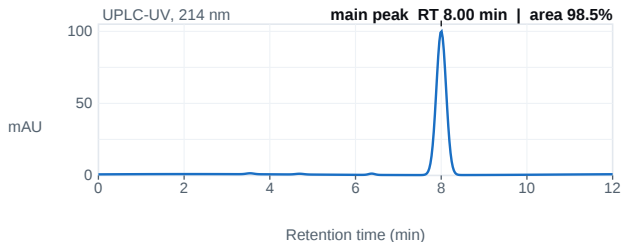
Fig. 1 — UPLC chromatogram; main peak 8.00 min, 98.5% area.
