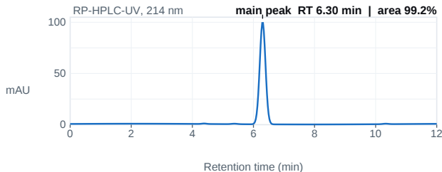
Fig. 1 — HPLC chromatogram; main peak 6.30 min, 99.2% area.
