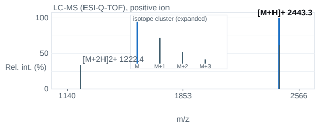
Fig. 2 — ESI-Q-TOF mass spectrum; base peak [M+H] + 2443.3 m/z.
