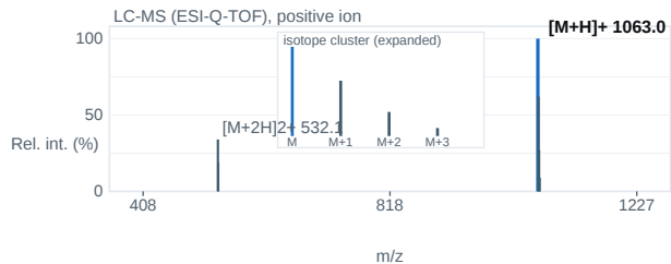
Fig. 2 — ESI-Q-TOF mass spectrum; base peak [M+H] + 1063.0 m/z.
