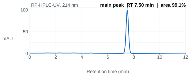
Fig. 1 — HPLC chromatogram; main peak 7.50 min, 99.1% area.
