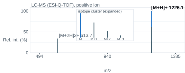
Fig. 2 — ESI-Q-TOF mass spectrum; base peak [M+H] + 1226.1 m/z.
