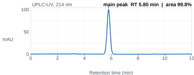
Fig. 1 — UPLC chromatogram; main peak 5.80 min, 99.8% area.
