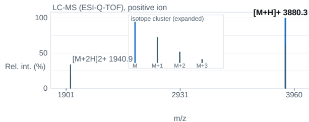
Fig. 2 — ESI-Q-TOF mass spectrum; base peak [M+H] + 3880.3 m/z.
