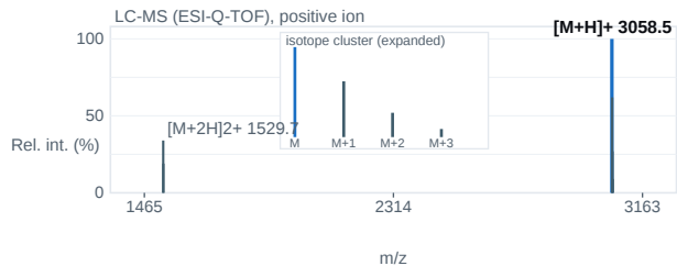
Fig. 2 — ESI-Q-TOF mass spectrum; base peak [M+H] + 3058.5 m/z.
