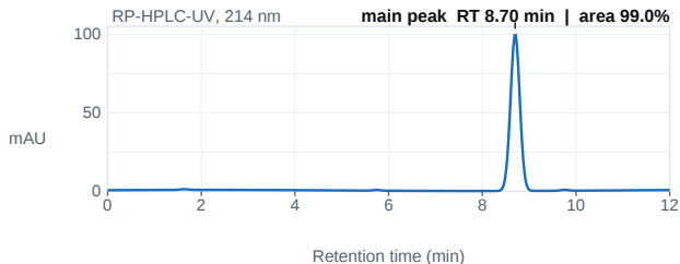
Fig. 1 — HPLC chromatogram; main peak 8.70 min, 99.0% area.
