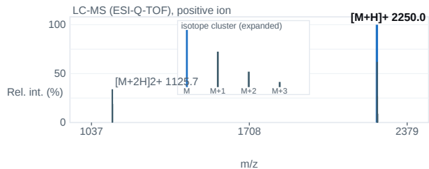
Fig. 2 — ESI-Q-TOF mass spectrum; base peak [M+H] + 2250.0 m/z.
