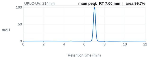
Fig. 1 — UPLC chromatogram; main peak 7.00 min, 99.7% area.
