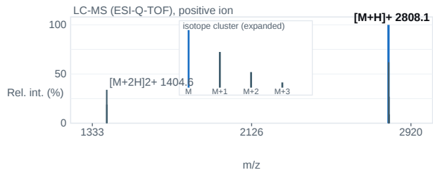
Fig. 2 — ESI-Q-TOF mass spectrum; base peak [M+H] + 2808.1 m/z.
