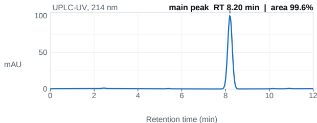
Fig. 1 — UPLC chromatogram; main peak 8.20 min, 99.6% area.
