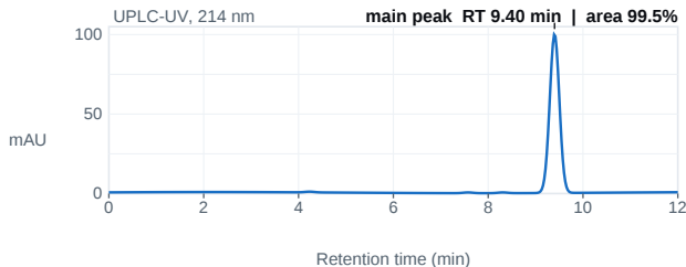
Fig. 1 — UPLC chromatogram; main peak 9.40 min, 99.5% area.
