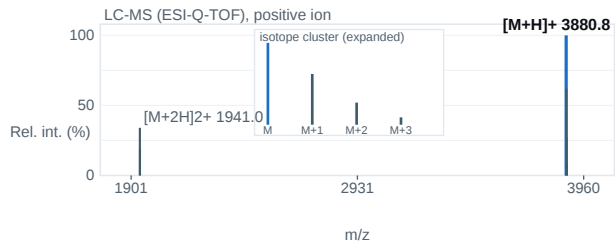
Fig. 2 — ESI-Q-TOF mass spectrum; base peak [M+H] + 3880.8 m/z.
