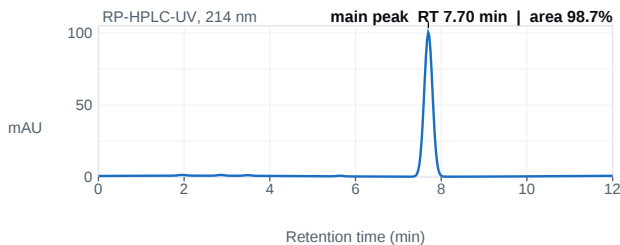
Fig. 1 — HPLC chromatogram; main peak 7.70 min, 98.7% area.
