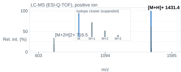
Fig. 2 — ESI-Q-TOF mass spectrum; base peak [M+H] + 1431.4 m/z.
