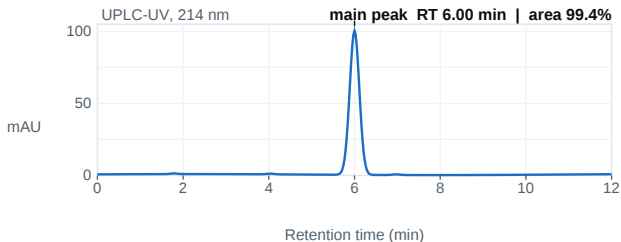
Fig. 1 — UPLC chromatogram; main peak 6.00 min, 99.4% area.
