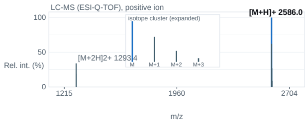
Fig. 2 — ESI-Q-TOF mass spectrum; base peak [M+H] + 2586.0 m/z.
