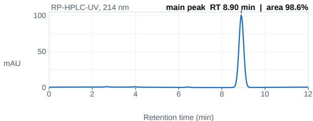
Fig. 1 — HPLC chromatogram; main peak 8.90 min, 98.6% area.
