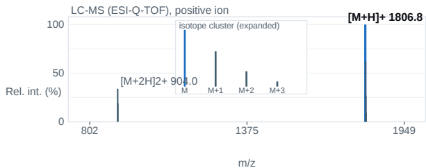
Fig. 2 — ESI-Q-TOF mass spectrum; base peak [M+H] + 1806.8 m/z.
