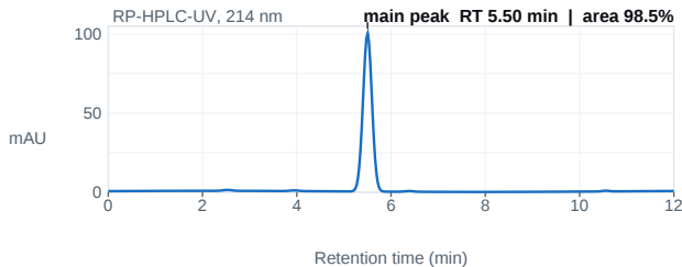
Fig. 1 — HPLC chromatogram; main peak 5.50 min, 98.5% area.
