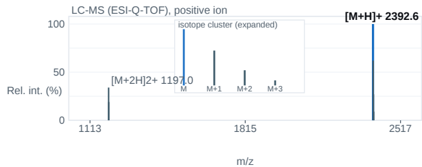
Fig. 2 — ESI-Q-TOF mass spectrum; base peak [M+H] + 2392.6 m/z.
