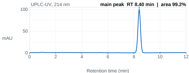
Fig. 1 — UPLC chromatogram; main peak 8.40 min, 99.2% area.
