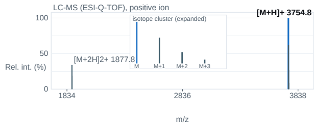
Fig. 2 — ESI-Q-TOF mass spectrum; base peak [M+H] + 3754.8 m/z.
